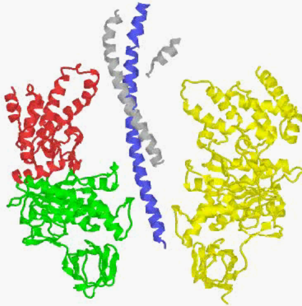
A cross-section view of alpha-beta-gamma By Hongyun Wang & George Oster, U.C.Berkeley
